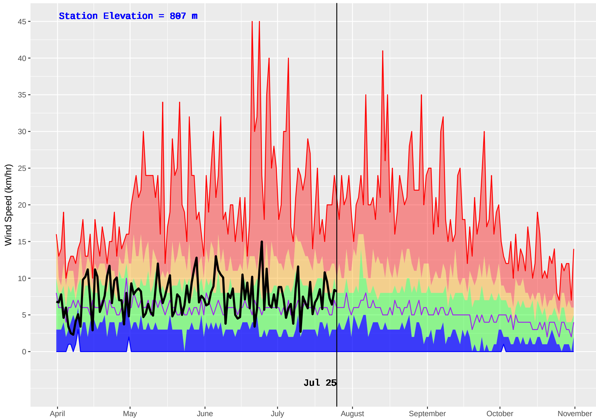
BEAVERDELL (390) : Historical (1970–2016) and Current (2018) Noon Wind Speed
