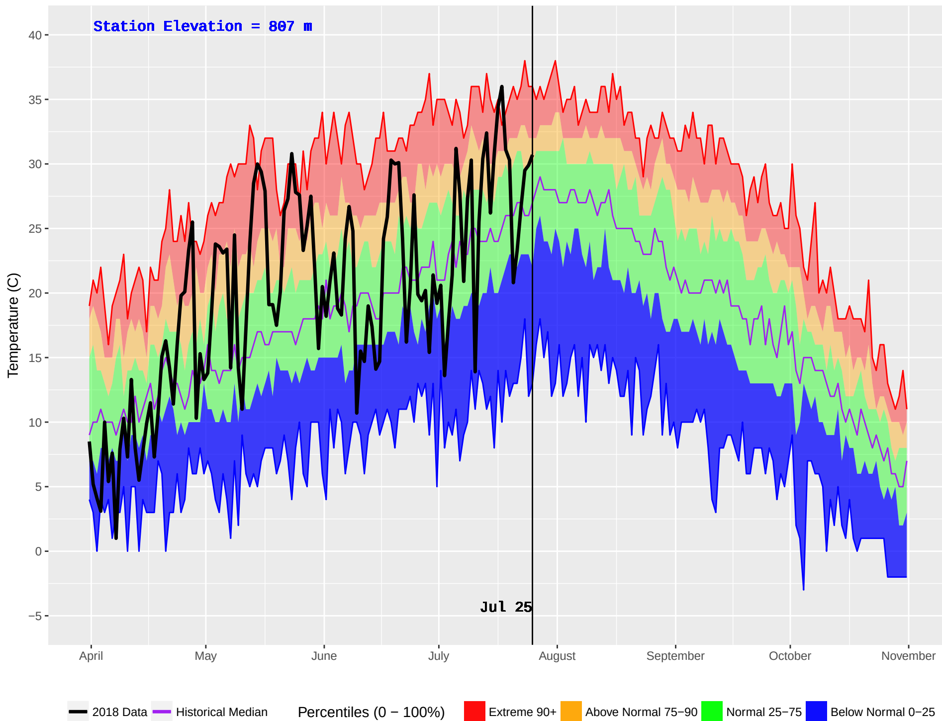
BEAVERDELL (390) : Historical (1970–2016) and Current (2018) Noon Temperature
